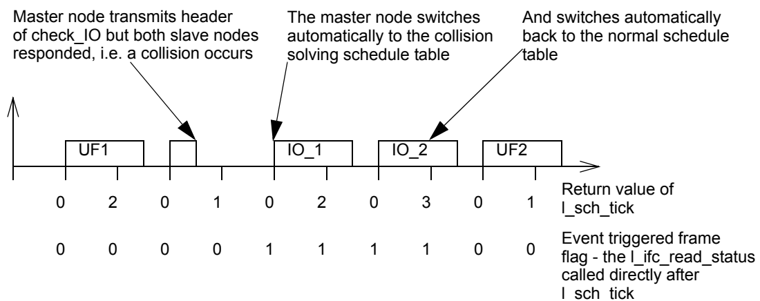
Figure 7.1: Event triggered frame collision solving example
